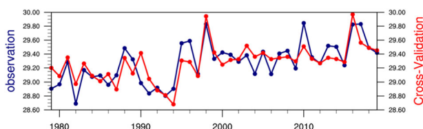
Fig. 5 Hindcast of the SWP SST-based prediction model. The observed (blue) and hindcasted (red) SST series (units: °C) of the TWP using the ten-fold cross-validation method (see Methods for details) for the period 1979–2019.
